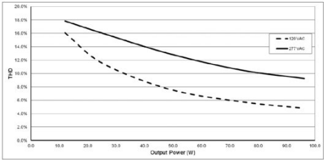
Typical THD
